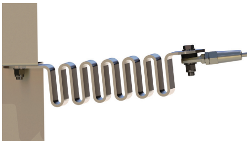
Overhead End Termination attached to Structure
