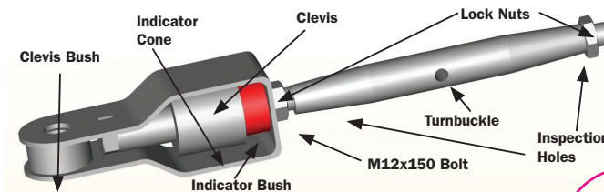
Figure 22 - Tension Indicator Assembly with Turnbuckle
